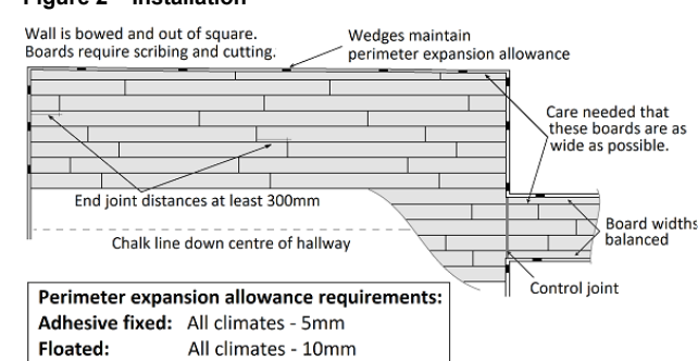
Figure 2 – Installation
