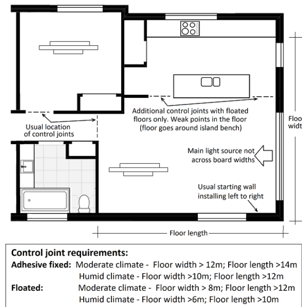
Figure 2 – Installation
