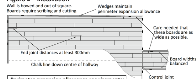
Figure 2 – Installation
